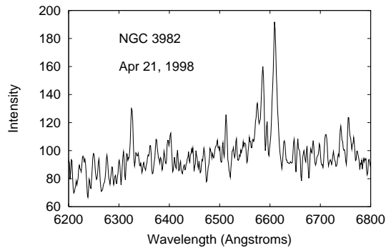
Fig. 5. Observed spectrum of the core of the host galaxy NGC 3982. The emission pattern around 6600 Å is due to H\alpha , [N II] and [S II].
